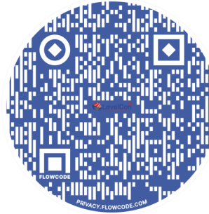
iOS App
