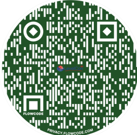
Android App
